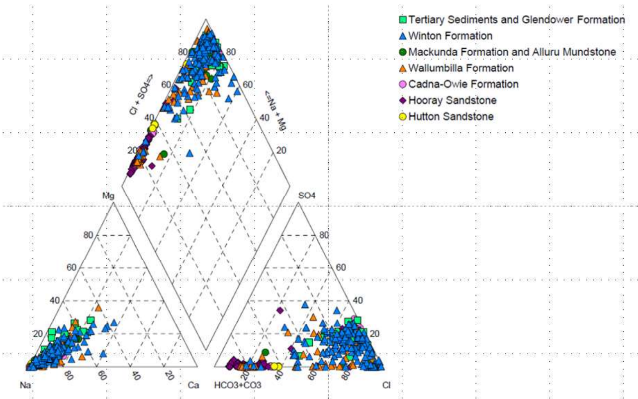
Figure 5.10 Piper Diagram of Groundwater Collected within the Project Area.
