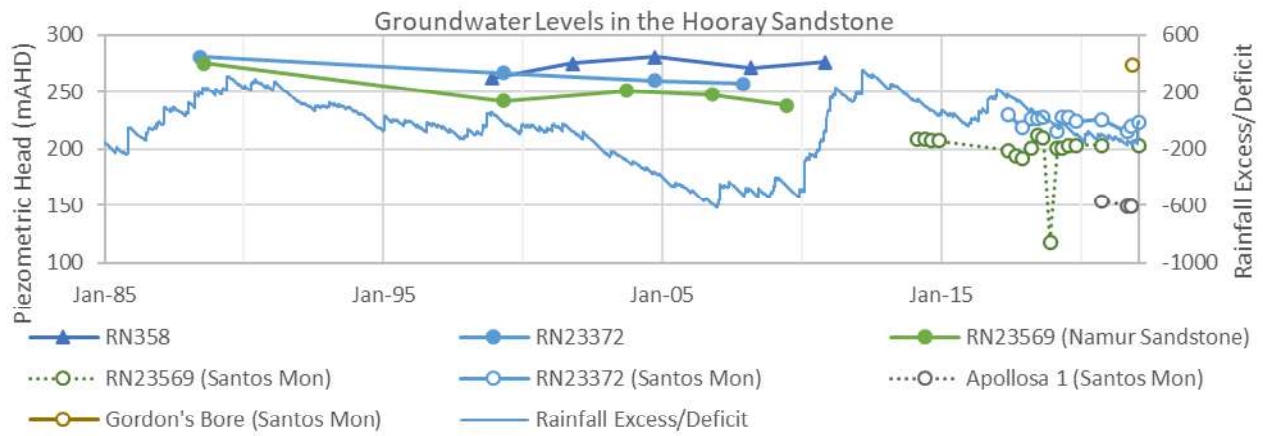
Figure 5.6 Available Water Level Data for GAB Monitoring Bores in the Hooray Sandstone
