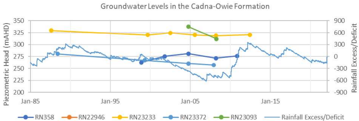
Figure 5.7 Available Water Level Data for GAB Monitoring Bores in the Cadna-Owie Formation
