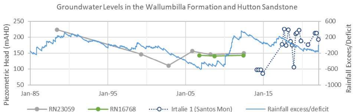
Figure 5.5 Available Data for Wallumbilla Formation and Hutton Sandstone Monitoring Bores
