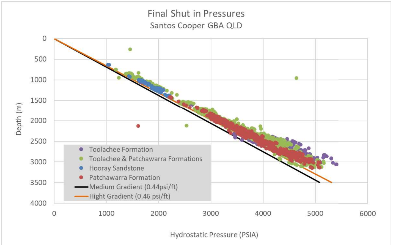
Figure 5.9 Final shut-in pressures from formation tests in Cooper Region
