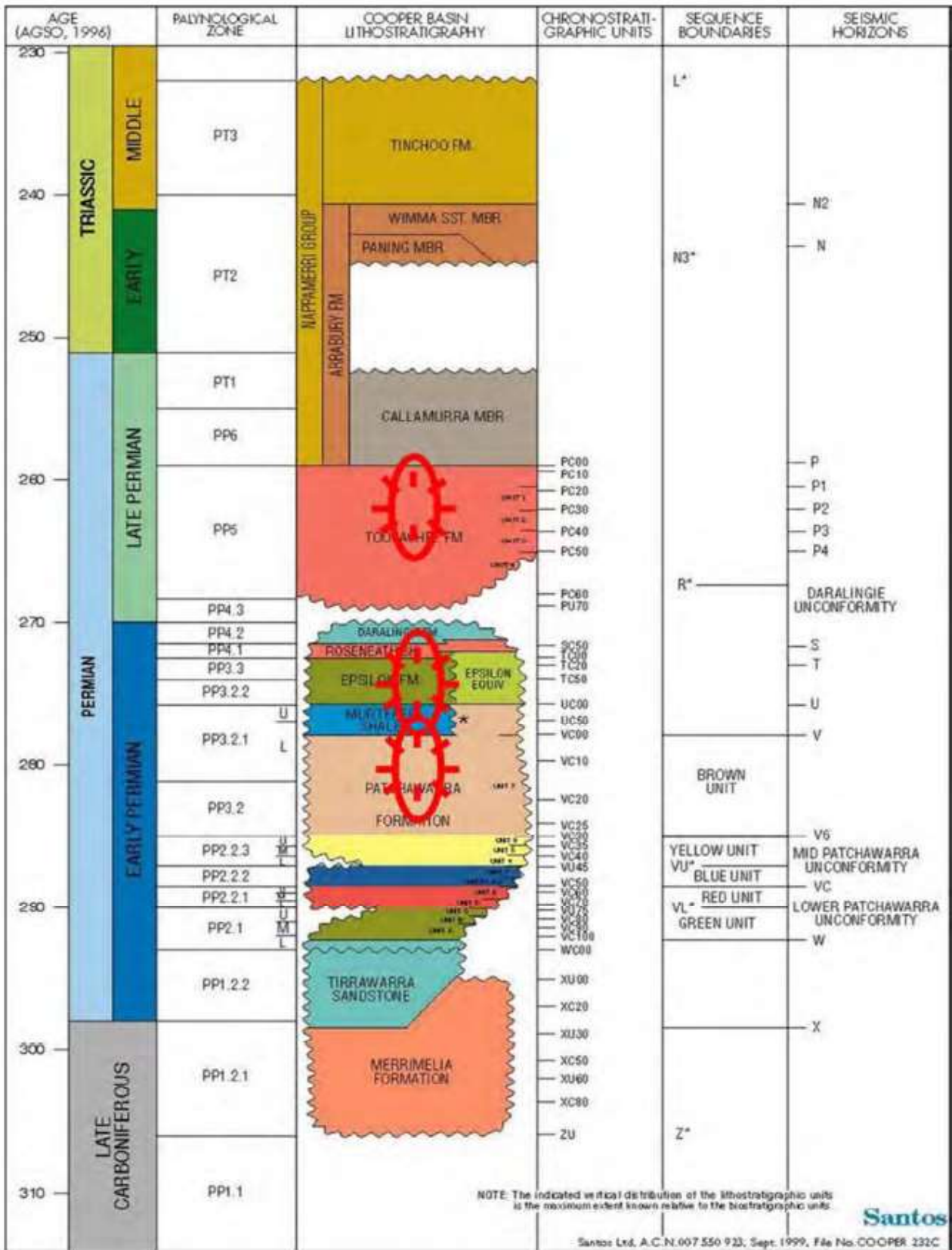
Figure 6.1 Gas Reservoirs Stratigraphic Distribution
