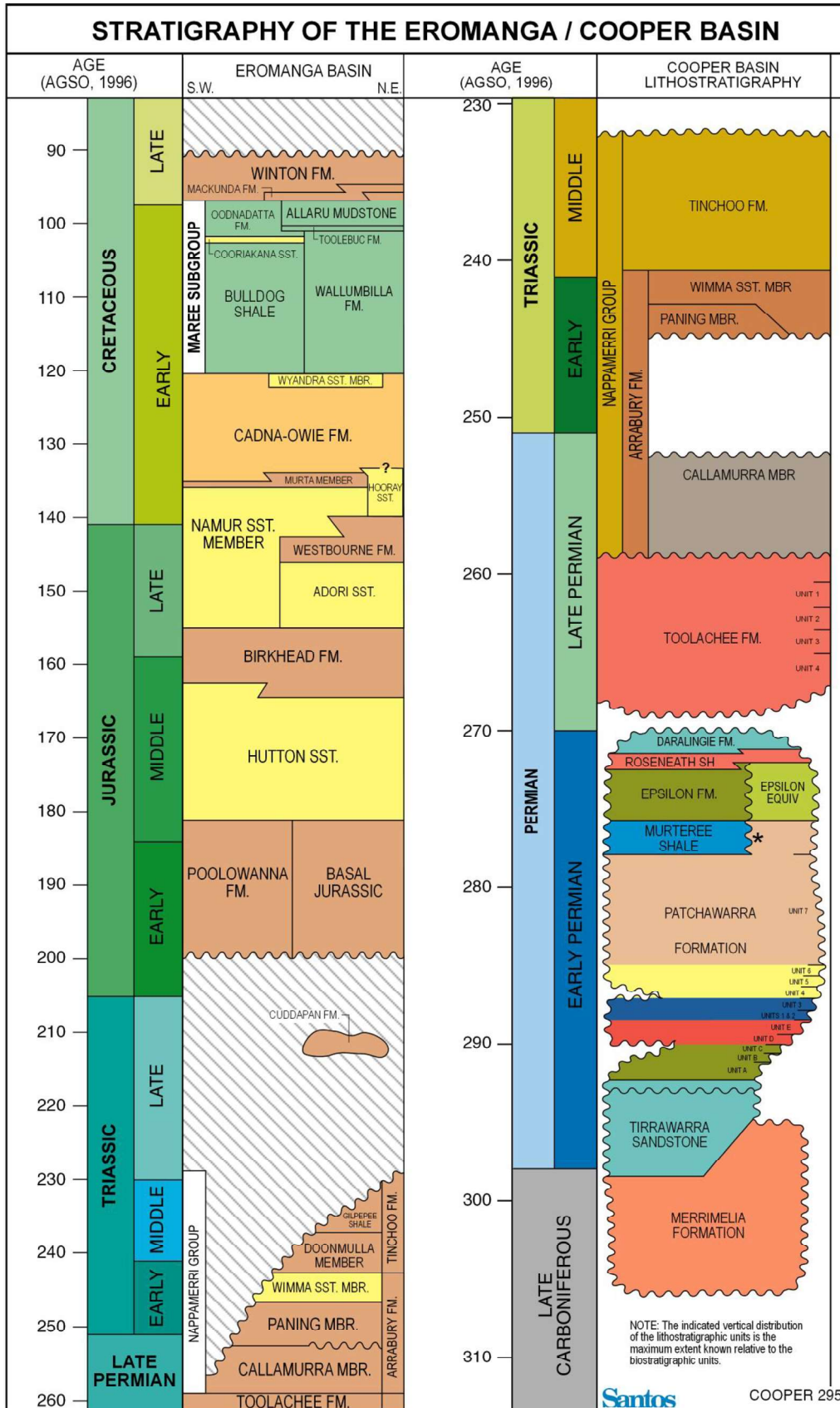
Figure 5.1 Regional Stratigraphy of the Cooper Basin
