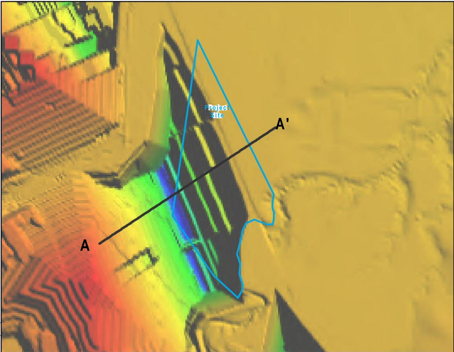
Profile A-A'
