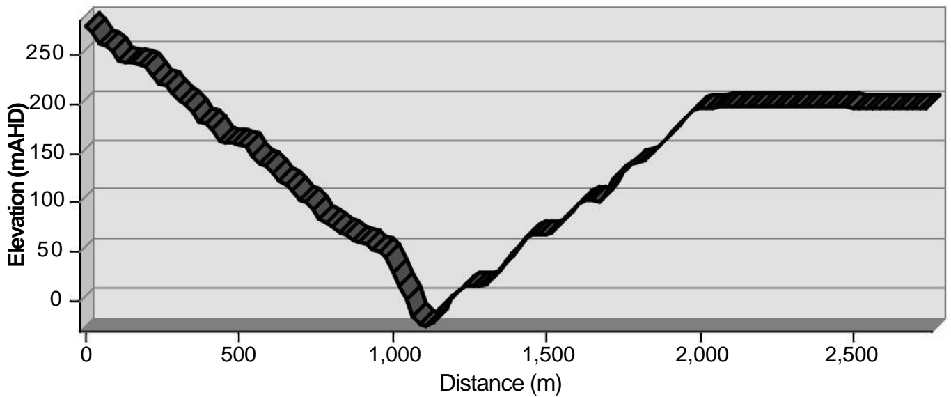
Profile A-A'
