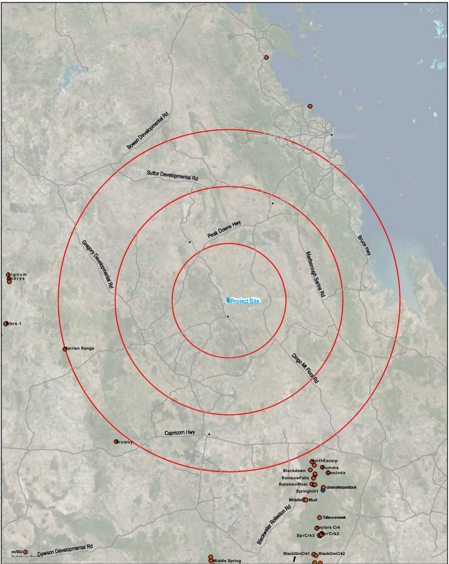
Figure 4 Registered Springs
