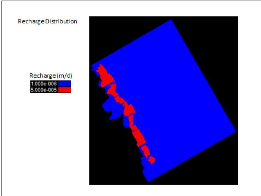
Figure 33 Recharge Distribution
