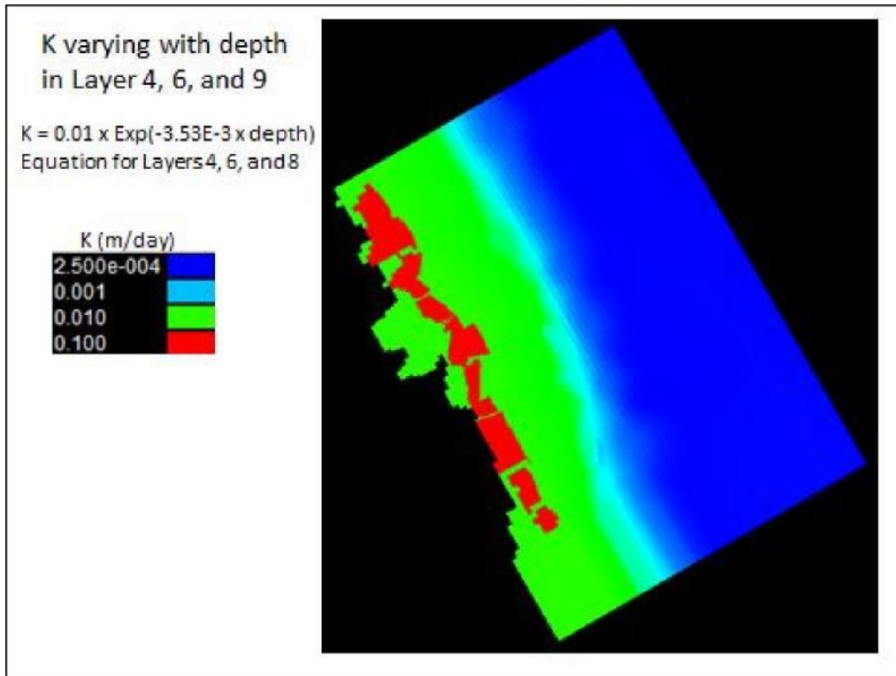
Figure 29 Hydraulic Conductivity (k) Distributions in Layer 4, 6, and 8
