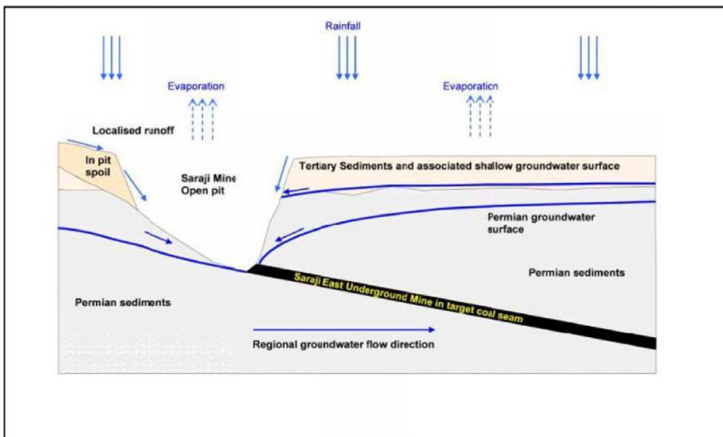
Figure 21 Conceptual Groundwater Model
