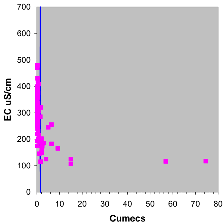
Figure A10: An actual plot of electrical conductivity (EC) against flow (cumeecs) at Utopia Downs in the Upper Dawson catchment. Vertical line on plot shows where data were initially separated into high and low flow conditions
