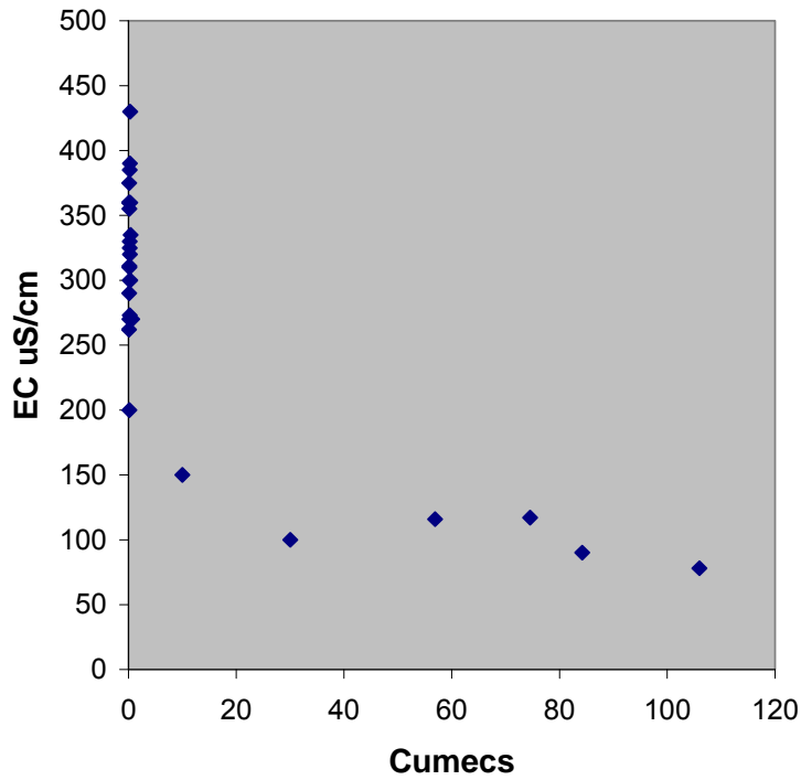
Figure A9: A conceptual relationship between electrical conductivity (EC) and flow (cumeecs) where EC decreases with high flow
