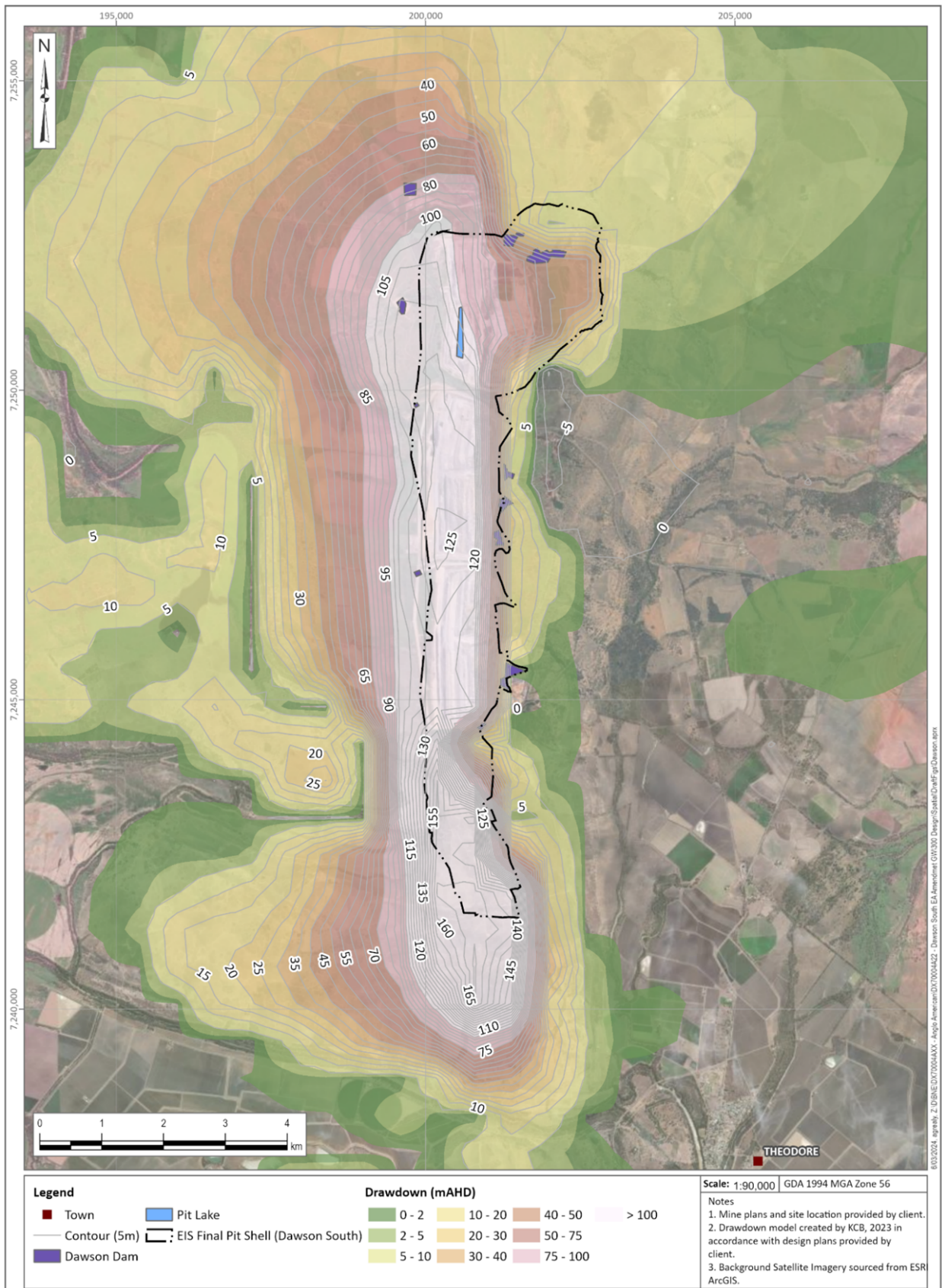
Figure I-9 Groundwater Drawdown 5 years, Existing mine plan - Post Design Closure
