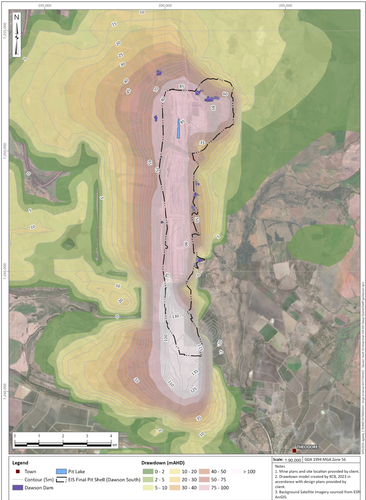
Figure I-12 Groundwater Drawdown 50 years Post-Closure, Proposed
