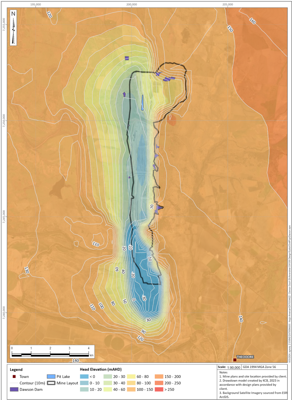
Figure I-5 Groundwater Elevation 5 years after End of Operations (Layer 2 Existing mine plan)
