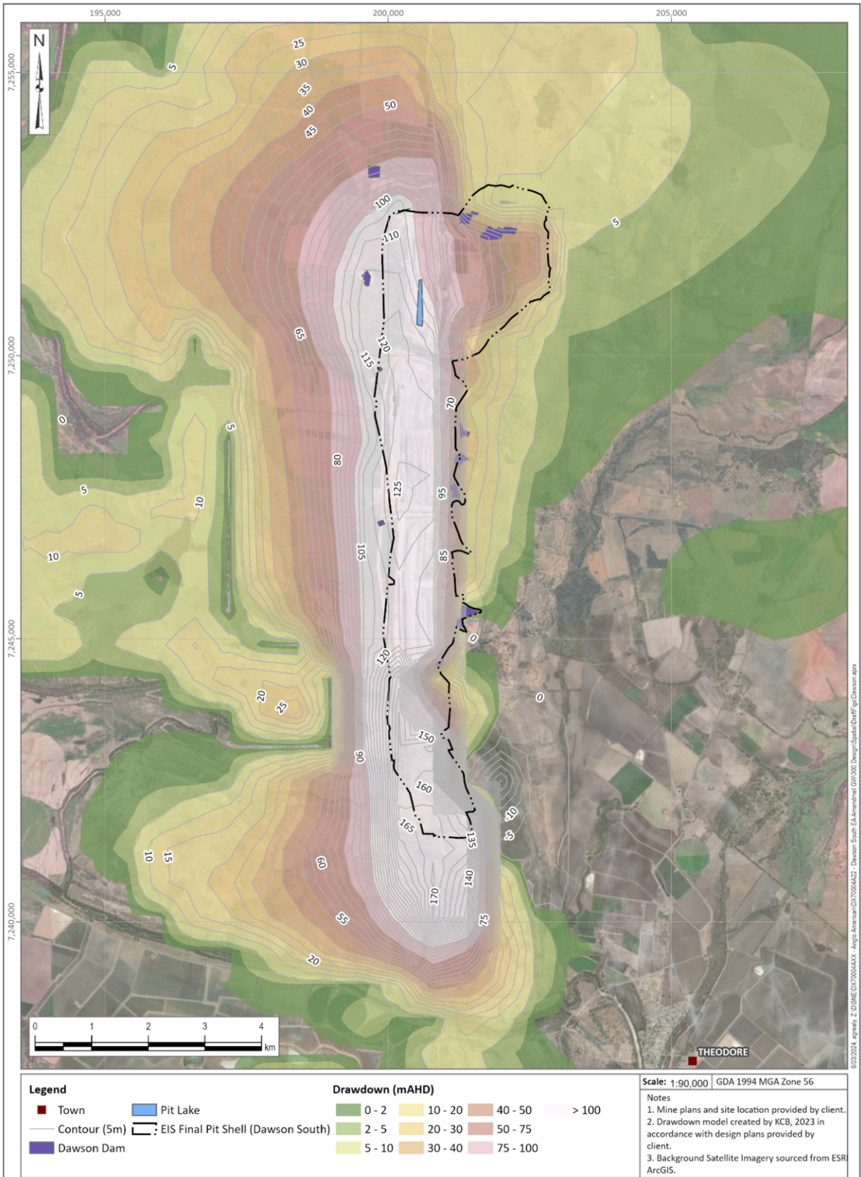
Figure I-10 Groundwater Drawdown 5 years, Proposed - Post Design Closure (Conservative)
