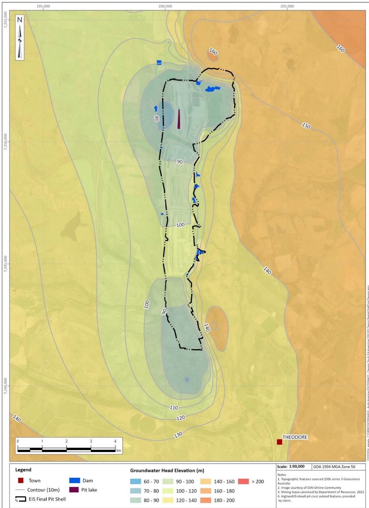
Figure I-8 Groundwater Elevation – 1000 year Post-Closure Design (Layer 2 Proposed)
