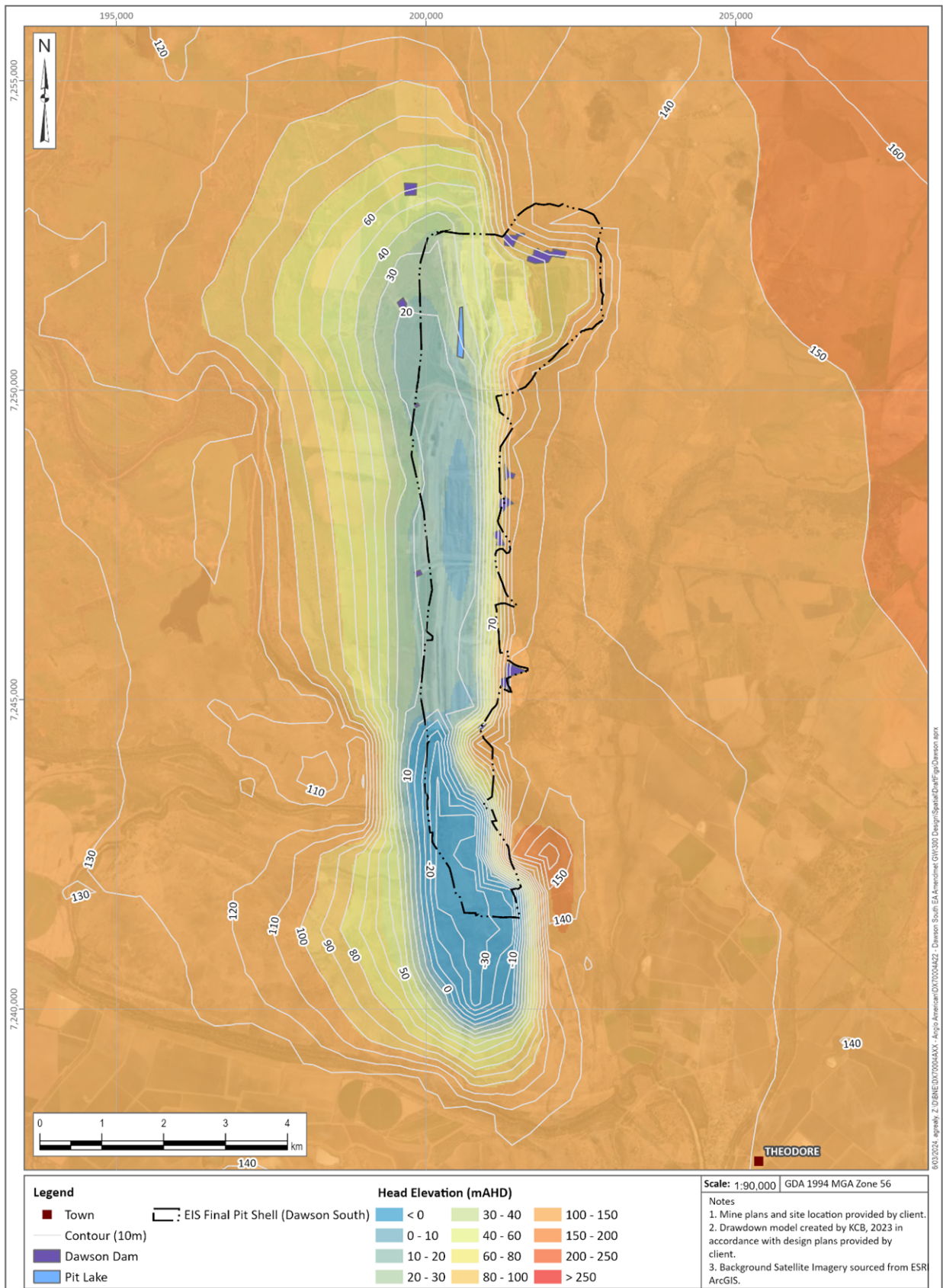
Figure I-6 Groundwater Elevations 5 years after End of Operations (Layer 2 Proposed)
