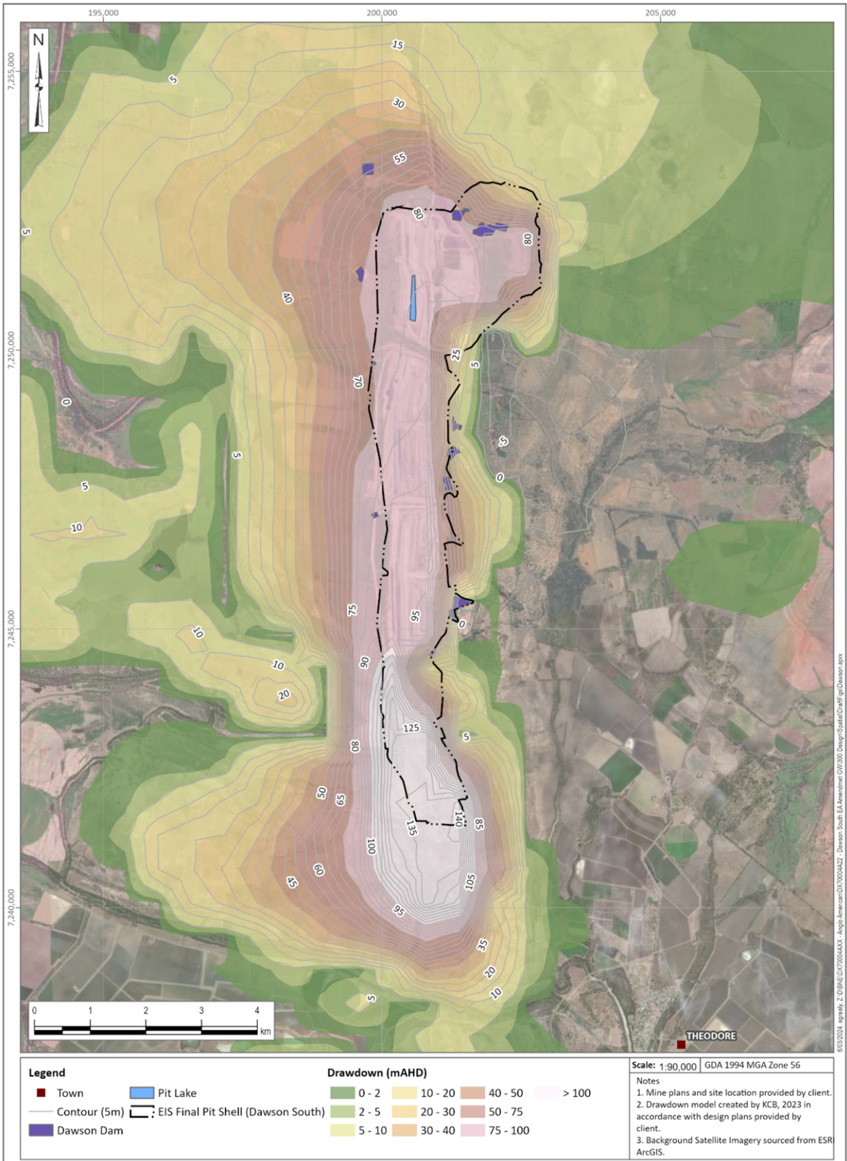
Figure I-11 Groundwater Drawdown 50 years Post-Closure- Existing mine plan
