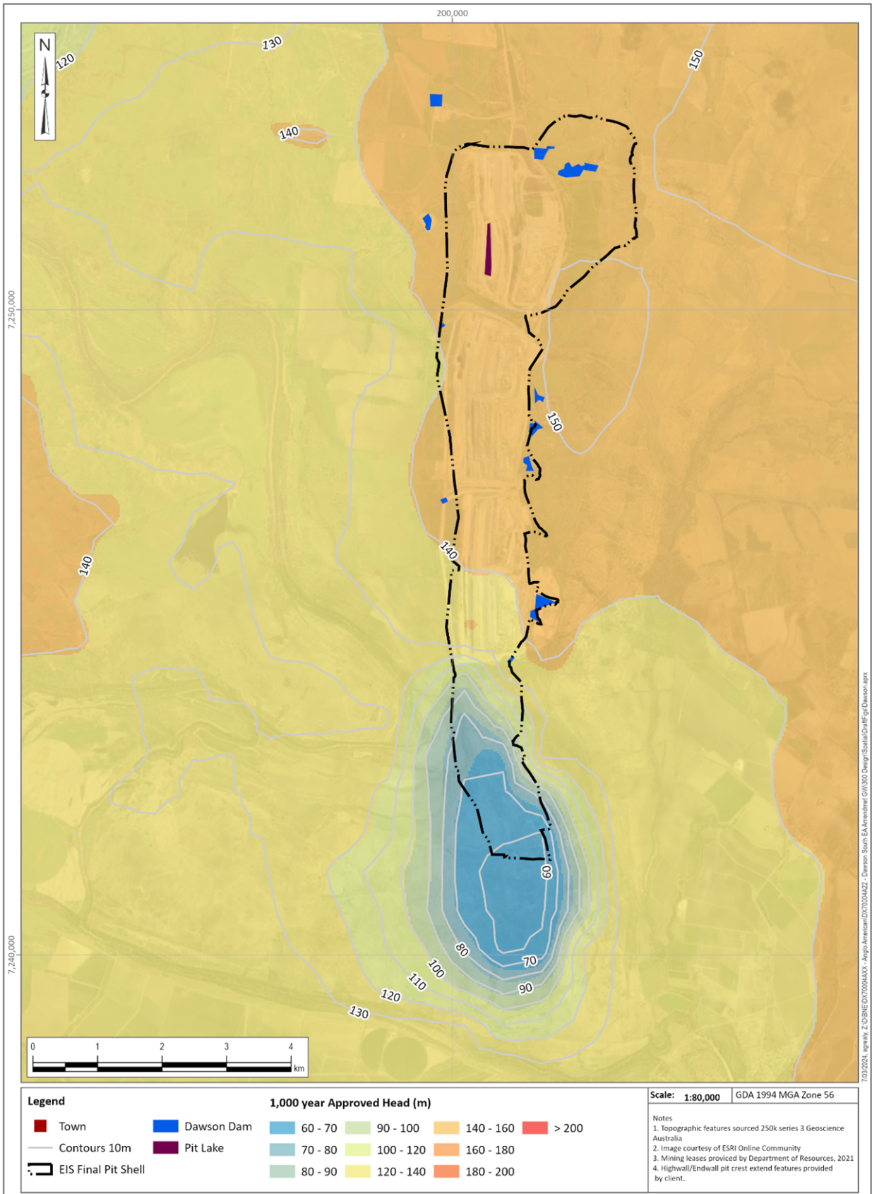
Figure I-7 Groundwater Elevation – 1000 year Post-Closure Design (Layer 2 Existing mine plan)
