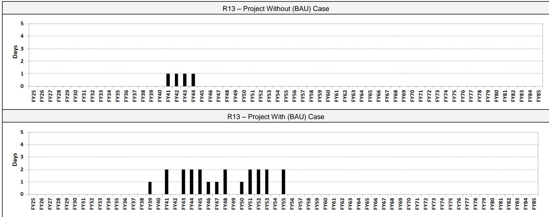
Figure 19: R13 Annual Variation in Predicted Exceedance Days over the LOM
