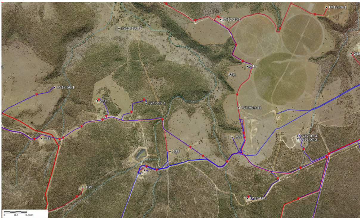
Figure 3 – Example LPD locations (Fairview Field)
