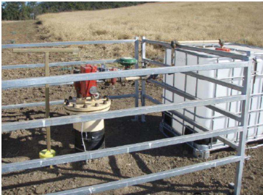
Figure 8 – Example LPD with Collection IBCs
