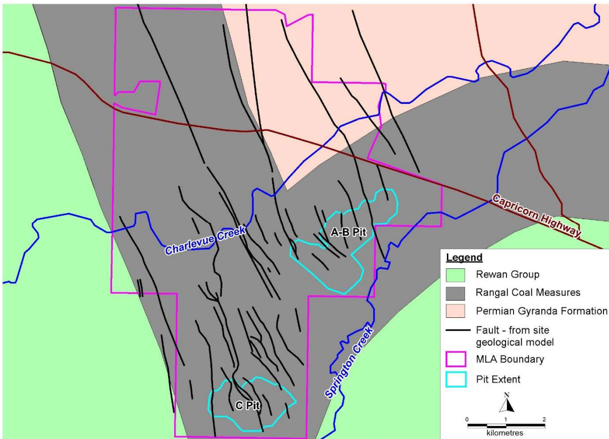
Figure 2-2: Solid Geology
