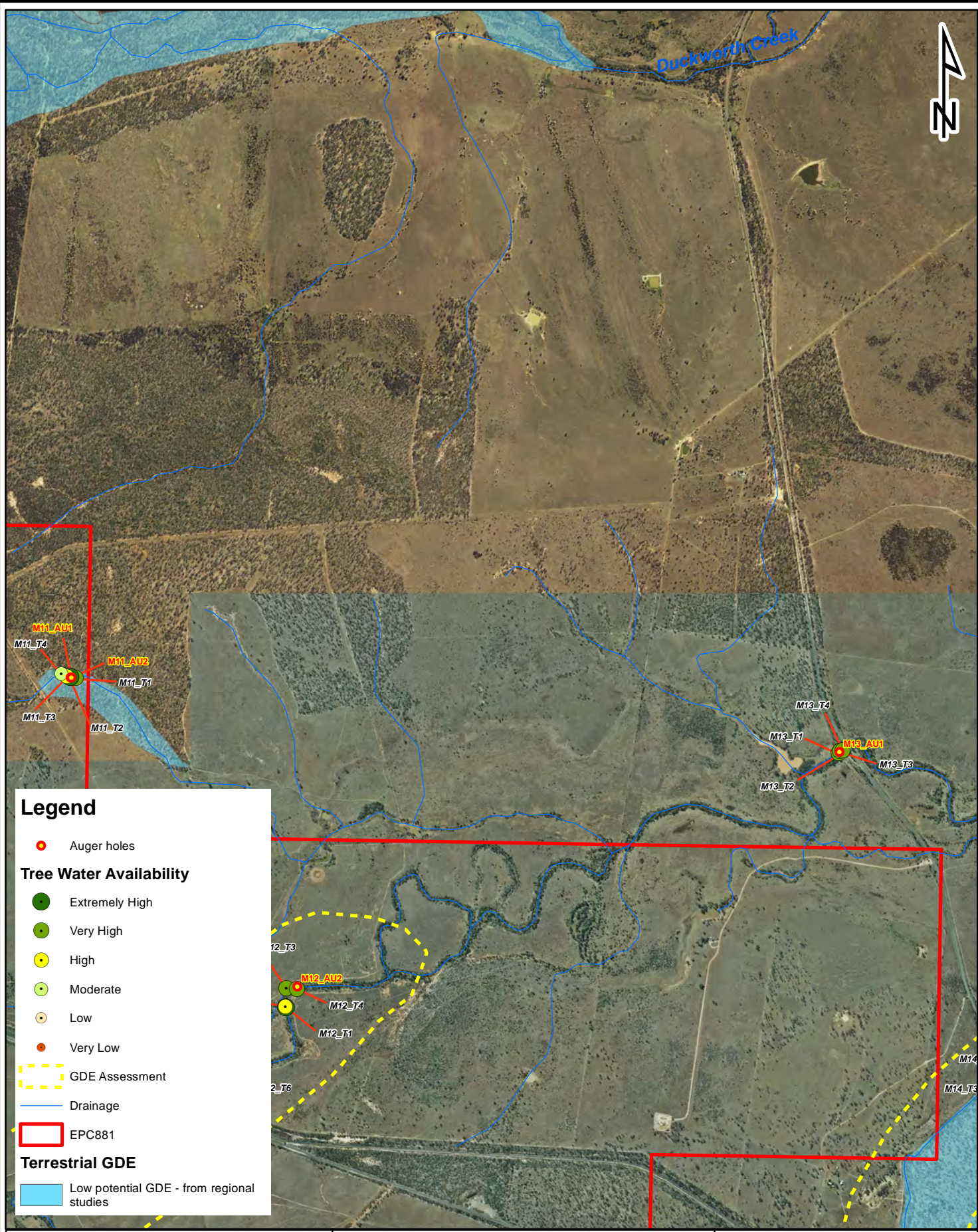
Figure 18. Tree water availability at Site M11 and M13 on Charlevue Creek and minor tributary
